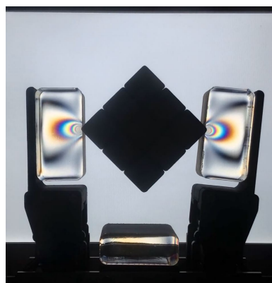
Fig. 15 A robot hand composed of photoelastic bodies
