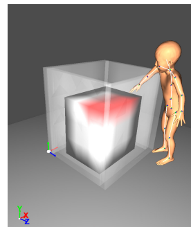
Fig. 23 Reachability-based Injury Risk Visualization
