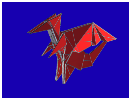
Fig. 25 Origami Simulator
